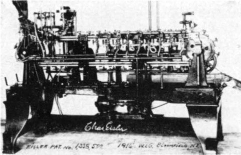
The first conveyor-type stem machine, designed by Eisler in 1916. The patent (No. 1,338,500) was assigned to Westinghouse in 1920.
